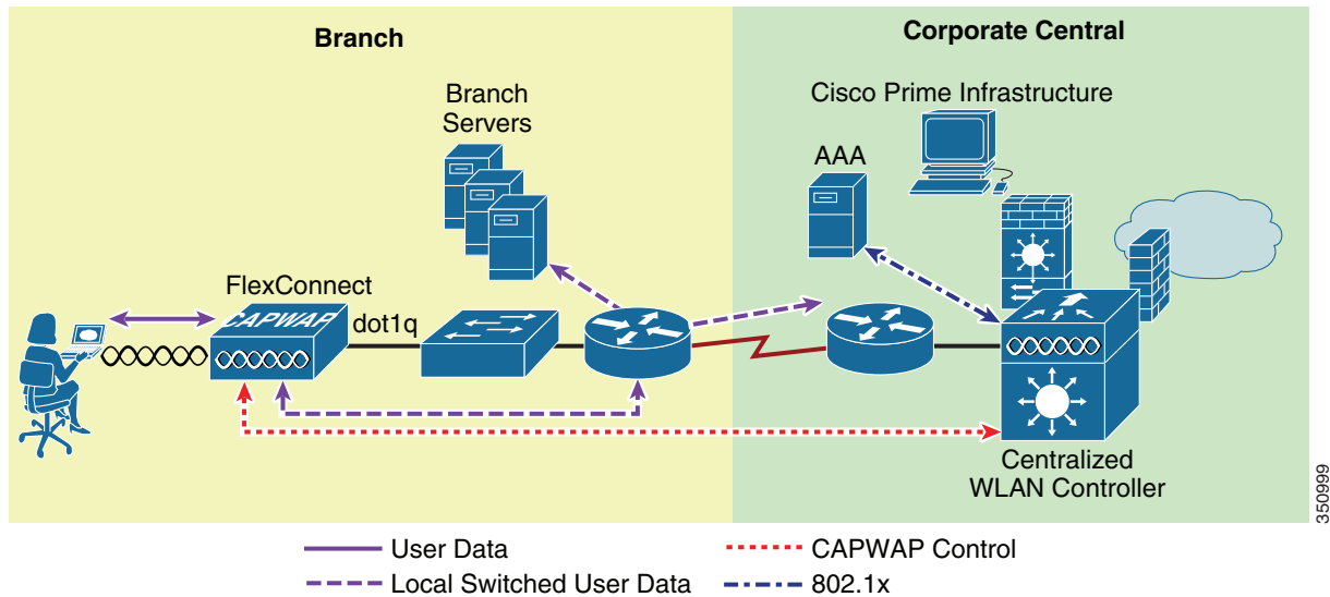
Figure 7-3 Authentication-Central/Switch-Local WLAN
