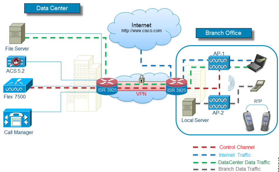
Figure 7-1 FlexConnect Architecture
