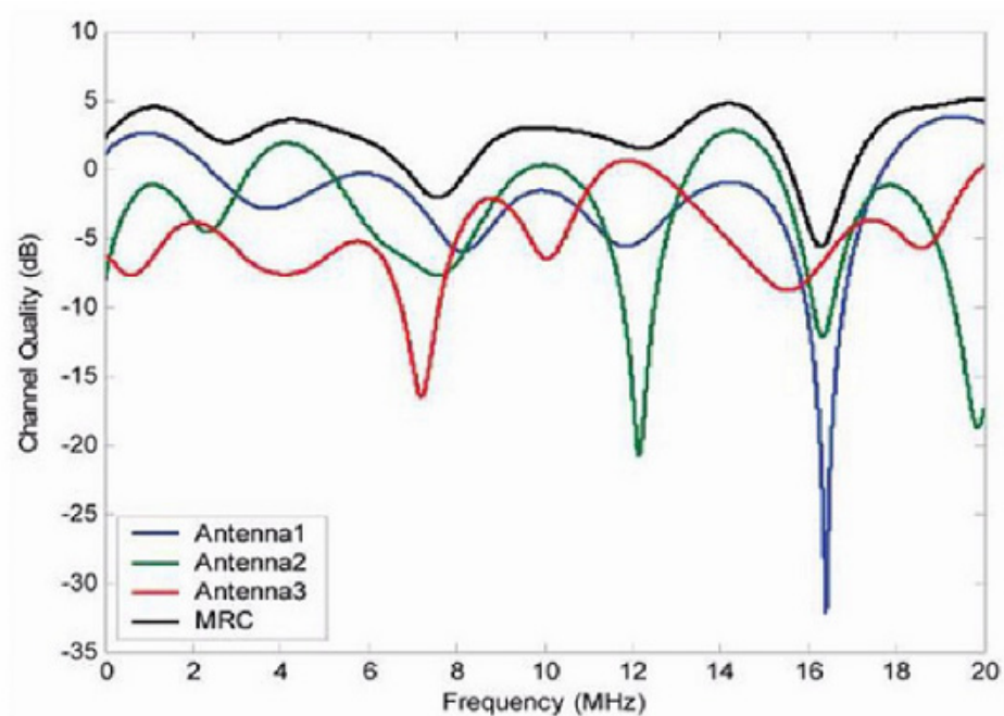
Figure 8-12 Reinforcement of Received Signal via MRC Algorithm
