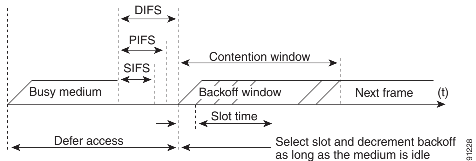
Figure 5-3 Interframe Spaces
