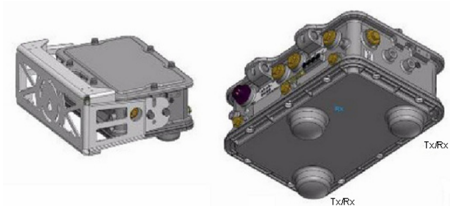
Figure 8-9 1552I Pole/Wall Mount
