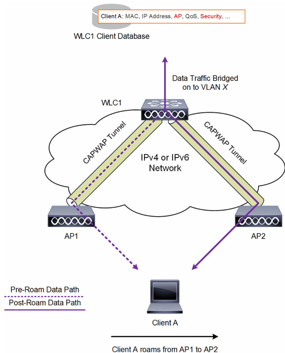
Figure 2-30 Intra-Controller Roaming
