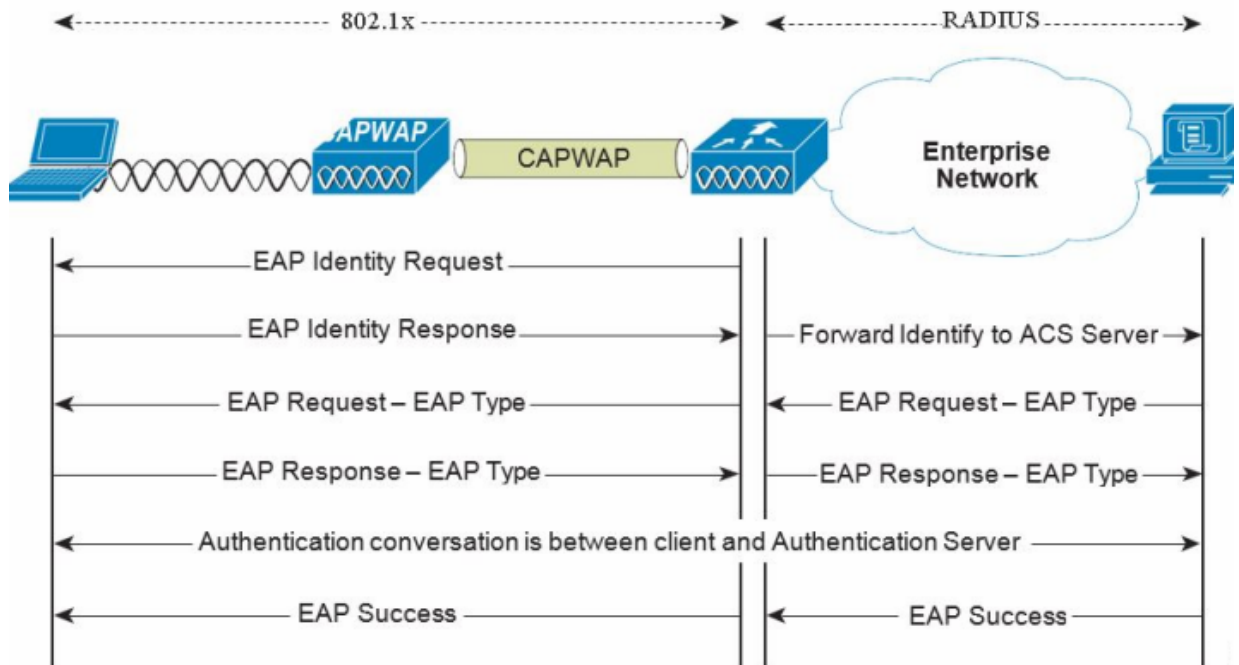
Figure 4-2 EAP Protocol Flow
