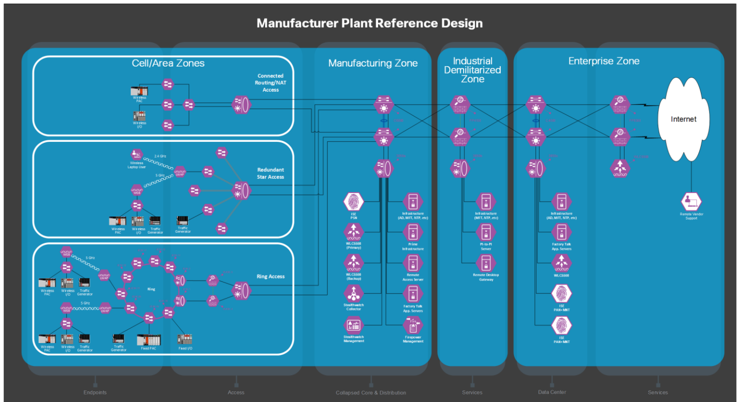
Figure 14 – Manufacturer Plant Reference Design
