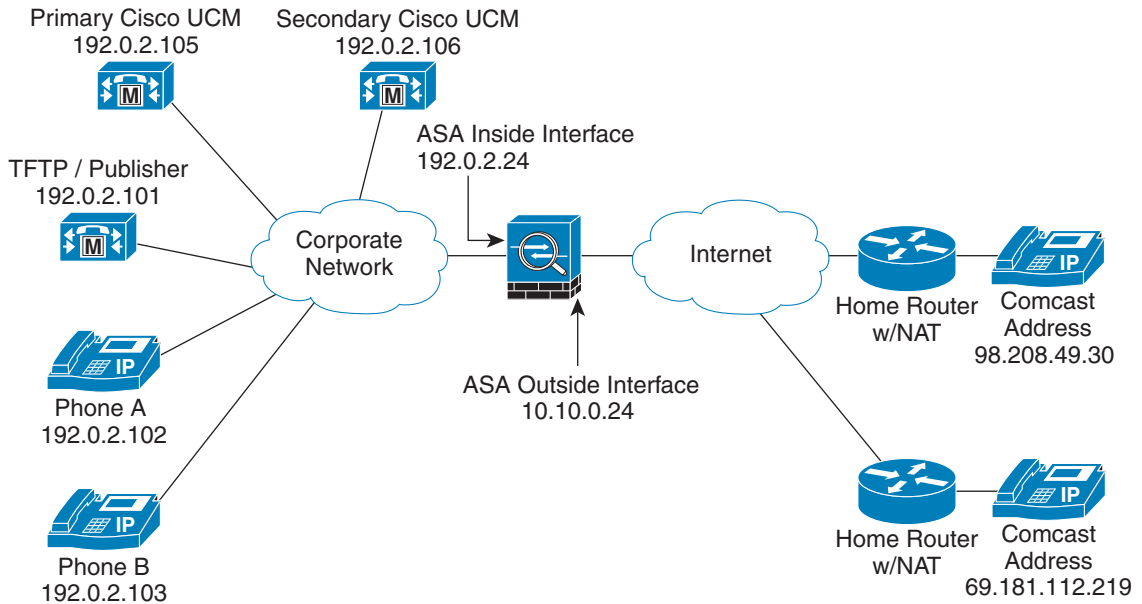
Figure 46-5 Mixed-mode Cisco UCM cluster, Primary Cisco UCM, Secondary Cisco UCM, and TFTP Server on Different Servers
