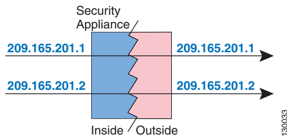
Figure 31-1 Identity NAT
