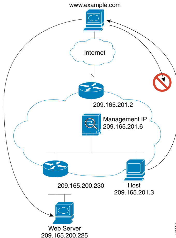
Figure 4-7 Typical Transparent Firewall Data Path
