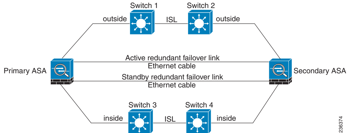
Figure 32-6 Connecting with Ethernet Cables
