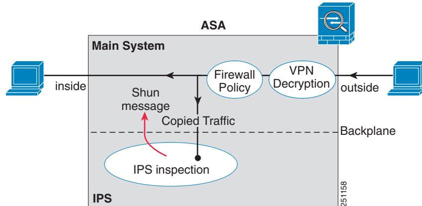
Figure 59-2 IPS Module Traffic Flow in the Adaptive Security Appliance: Promiscuous Mode
