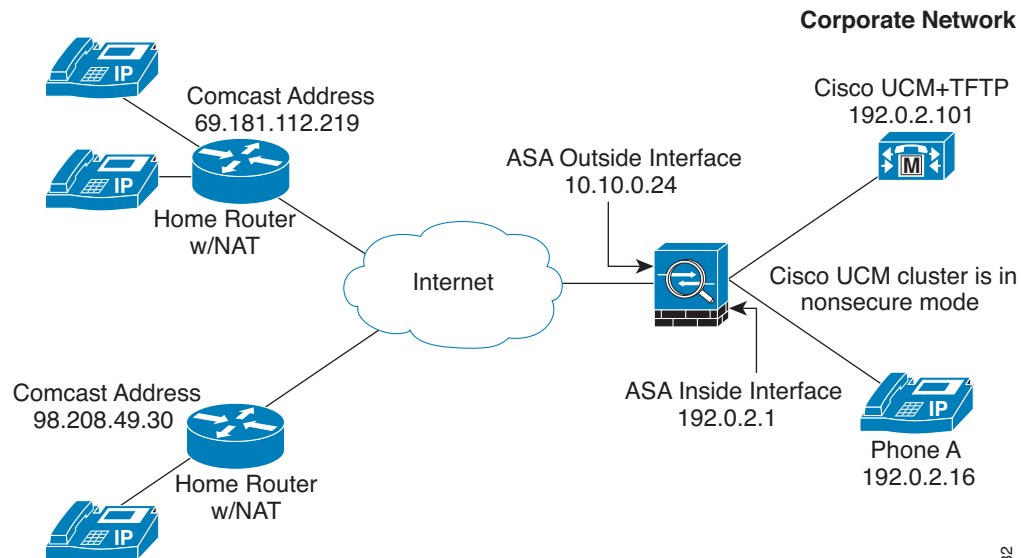
Figure 46-3 Mixed-mode Cisco UCM cluster, Cisco UCM and TFTP Server on Publisher
