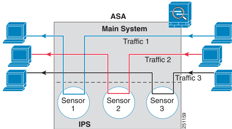
Figure 59-4 Single Mode Security Appliance with Multiple Virtual Sensors
