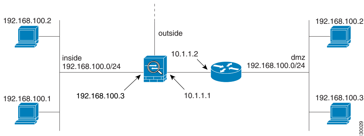
Figure 28-2 Using Outside NAT with Overlapping Networks
