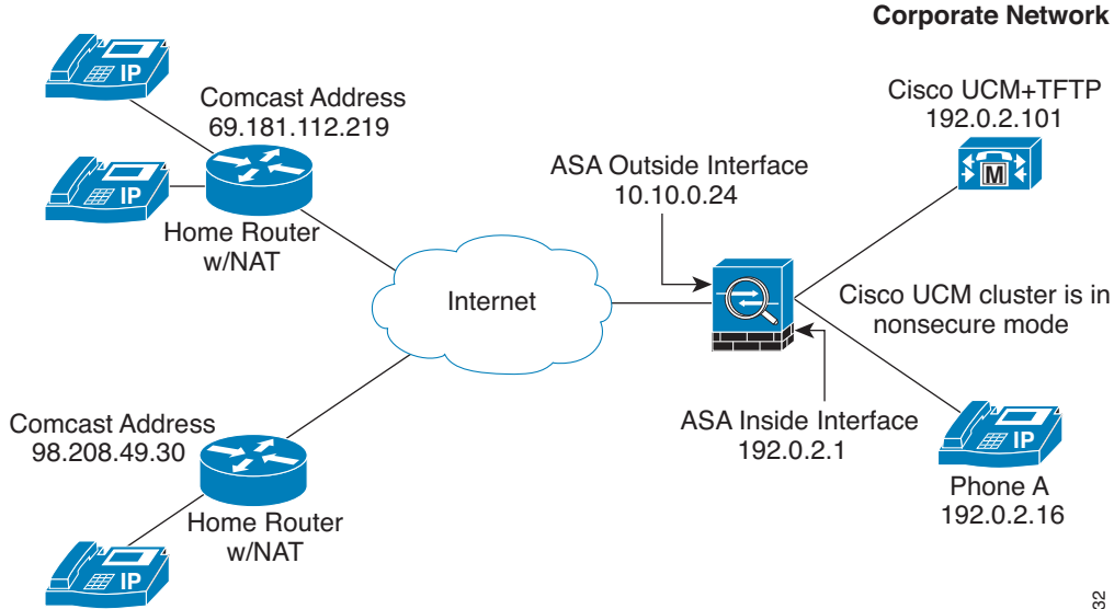
Figure 46-2 Nonsecure Cisco UCM cluster, Cisco UCM and TFTP Server on Publisher
