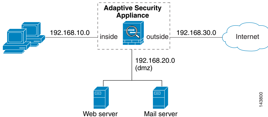
Figure 60-3 Common Network Configuration for CSC SSM Scanning
