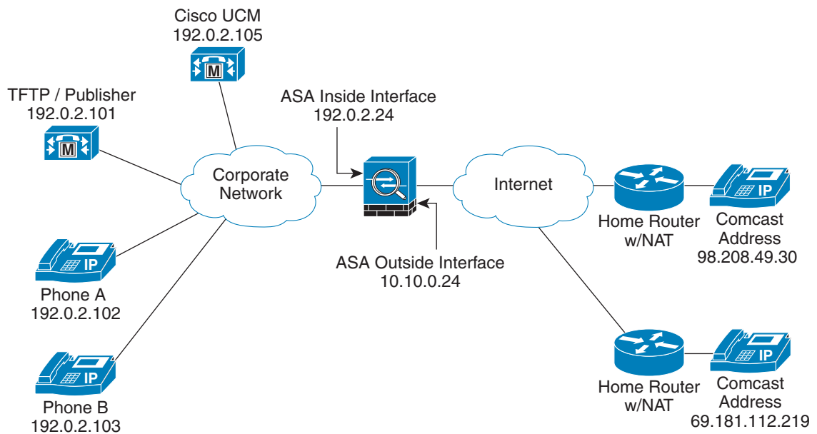
Figure 46-4 Mixed-mode Cisco UCM cluster, Cisco UCM and TFTP Server on Different Servers
