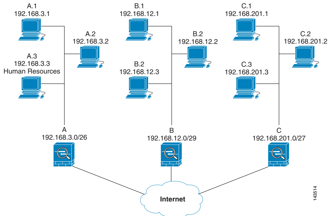
Figure 61-3 Effect of Permit and Deny ACEs on Traffic (Real Addresses)
