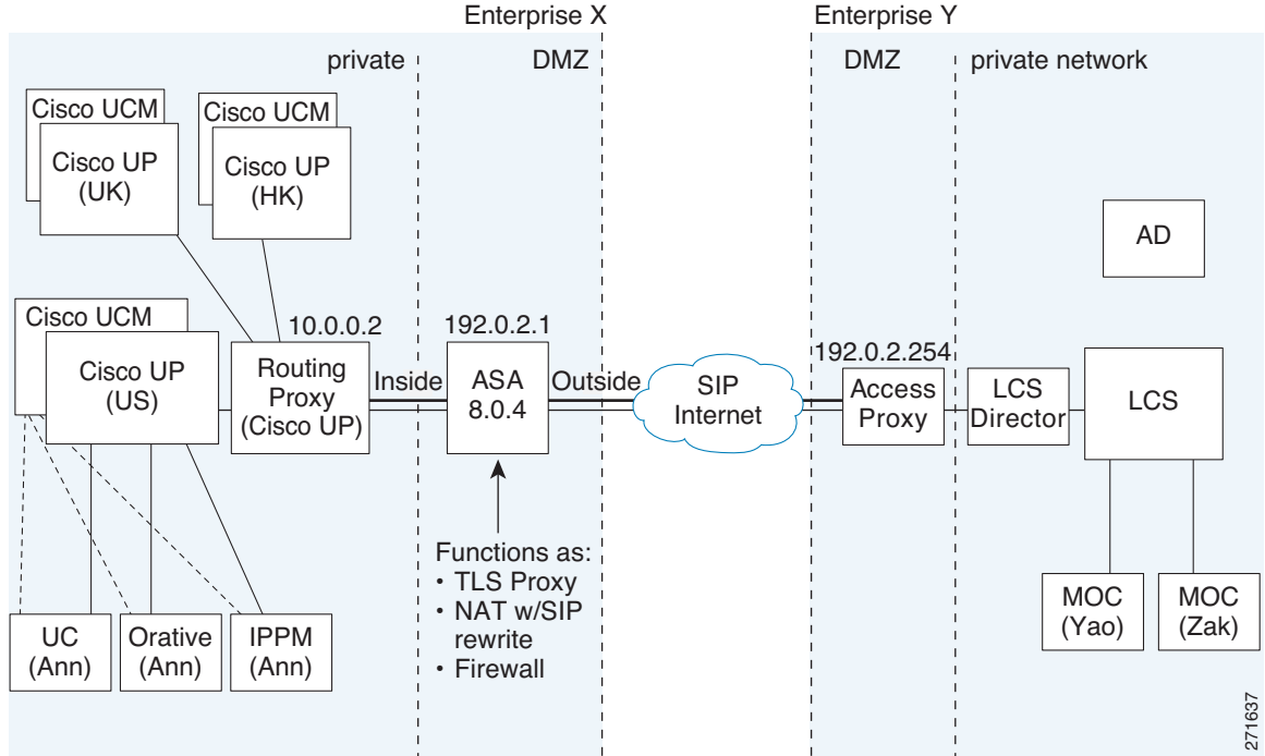
Figure 49-1 Typical Cisco Unified Presence/LCS Federation Scenario
