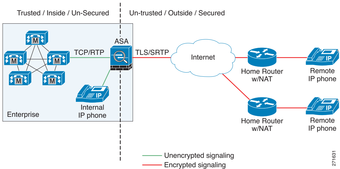
Figure 46-1 Phone Proxy Secure Deployment
