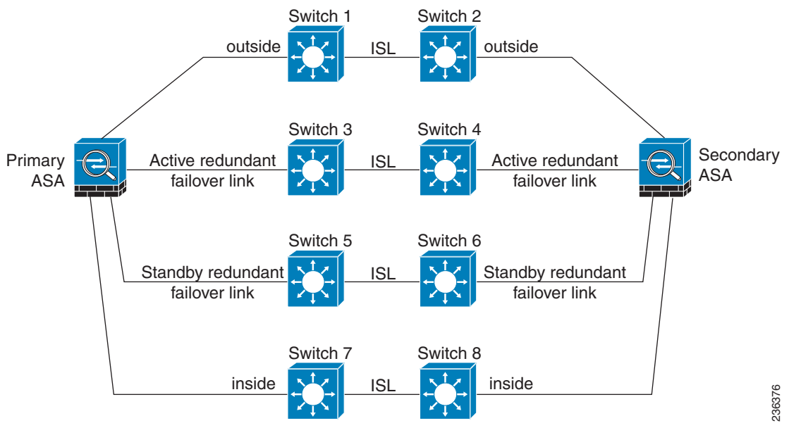
Figure 32-8 Connecting with Inter-switch Links
