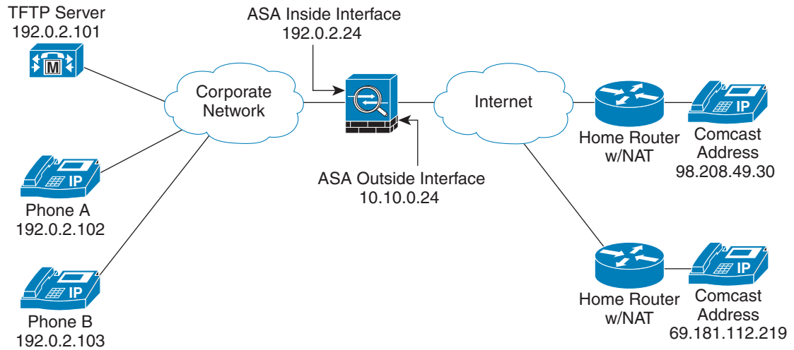
Figure 46-6 LSC Provisioning in Mixed-mode Cisco UCM cluster; Cisco UCM and TFTP Server on Publisher
