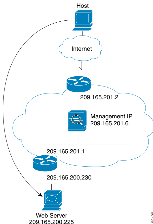
Figure 4-10 Outside to Inside
