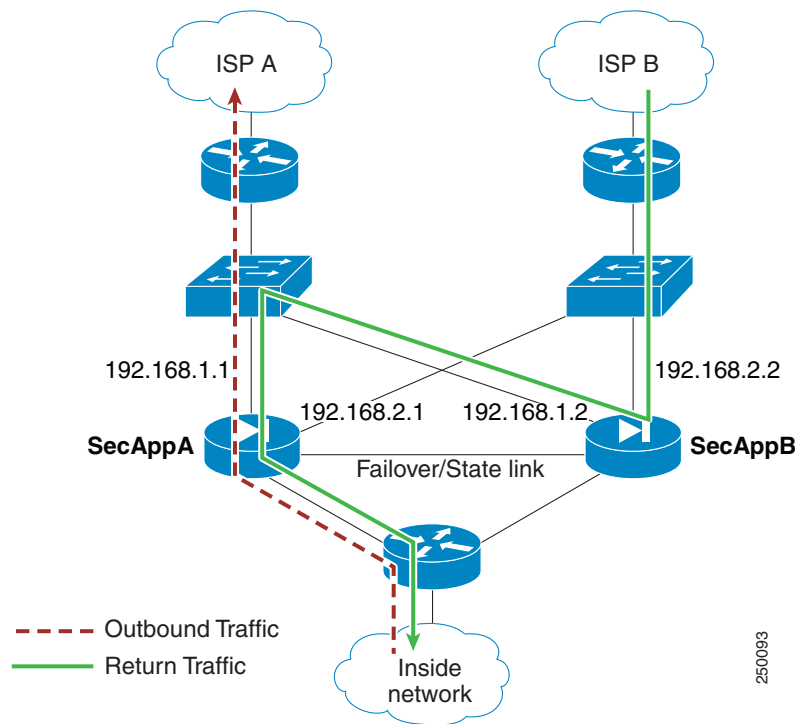
Figure 34-1 ASR Example
