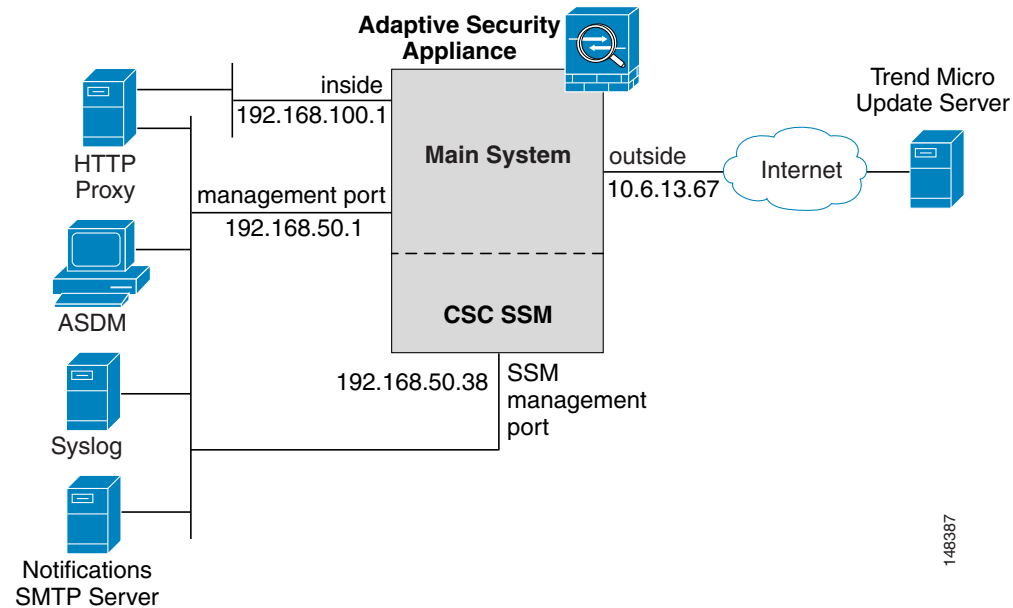
Figure 60-2 CSC SSM Deployment with a Management Network
