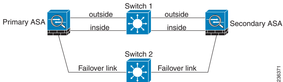
Figure 32-3 Connecting with a Different Switch
