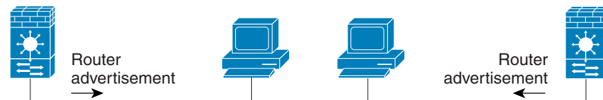
Figure 25-2 IPv6 Neighbor Discovery—Router Advertisement Message
