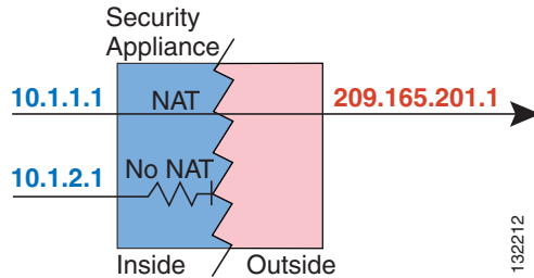
Figure 27-1 NAT Control and Outbound Traffic
