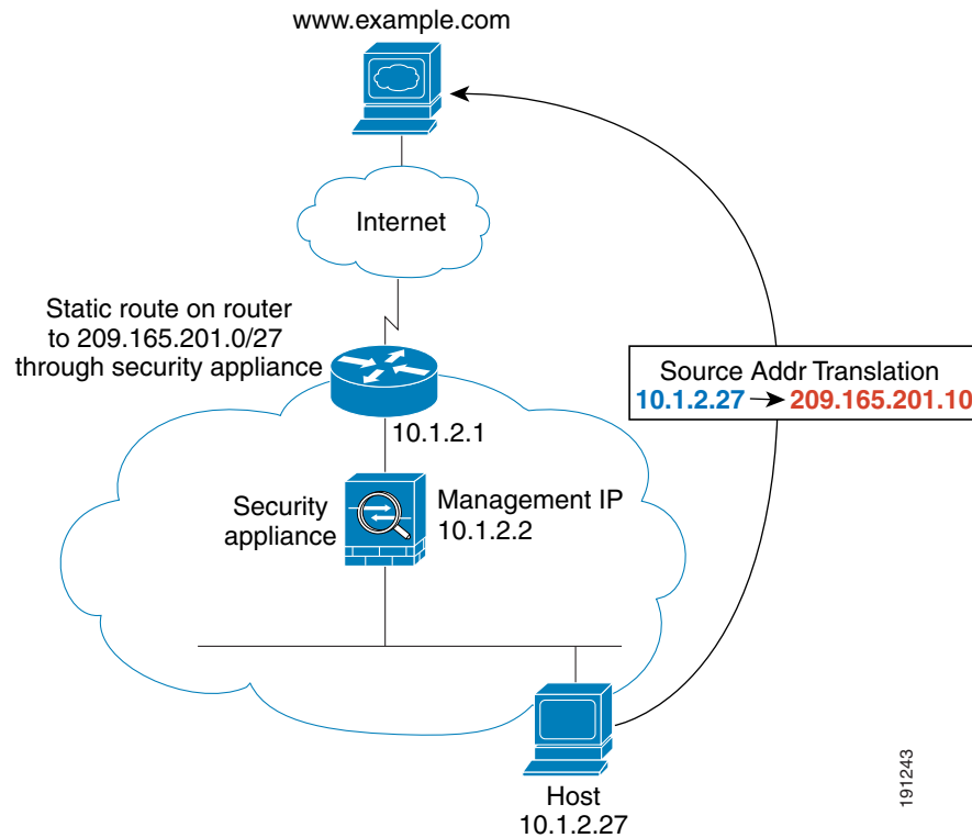
Figure 4-9 Inside to Outside with NAT
