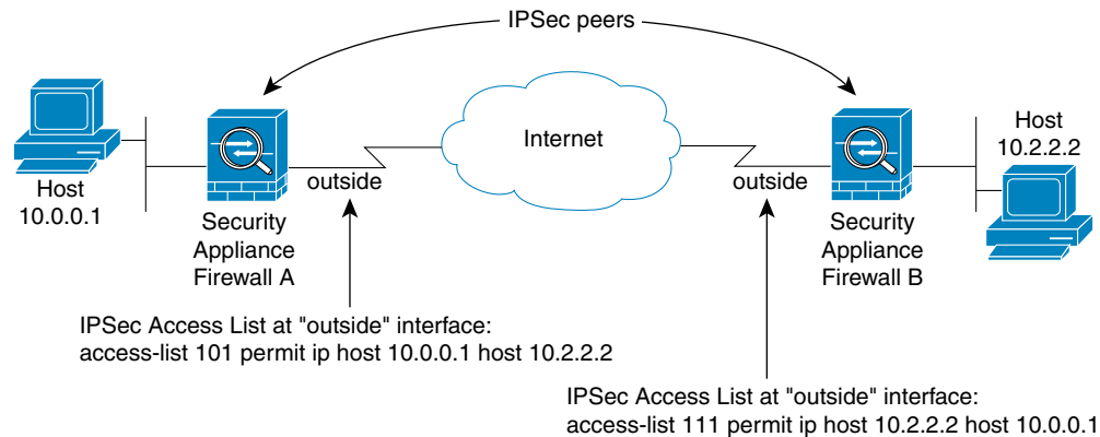
Figure 61-4 How Crypto Access Lists Apply to IPsec
