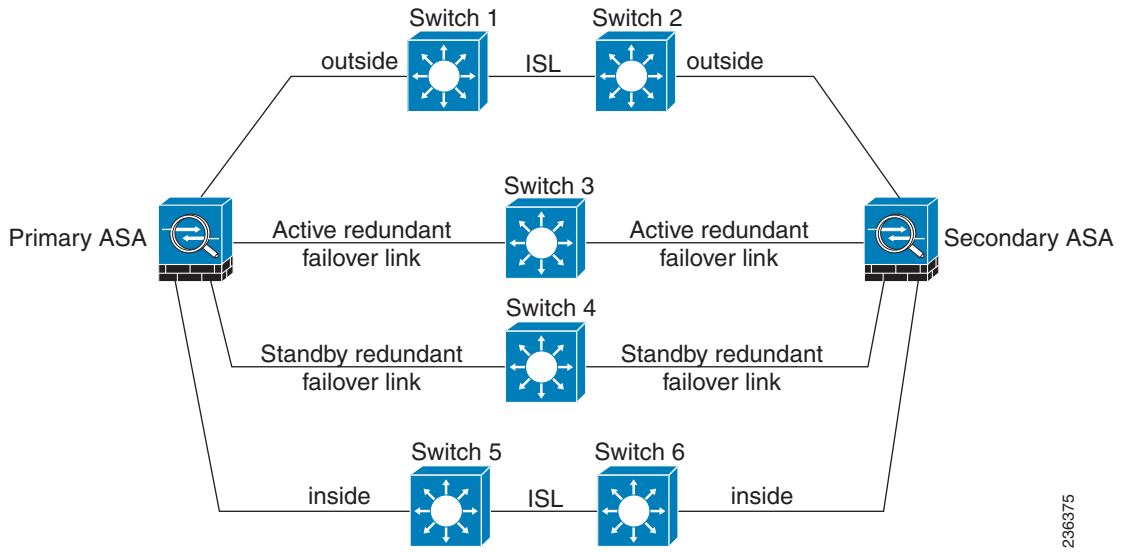
Figure 32-7 Connecting with Redundant Interfaces
