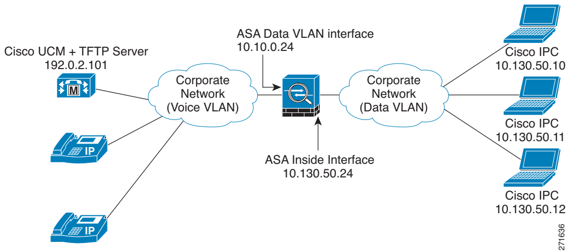
Figure 46-7 VLAN Transversal Between CIPC Softphones on the Data VLAN and Hard Phones on the Voice VLAN
