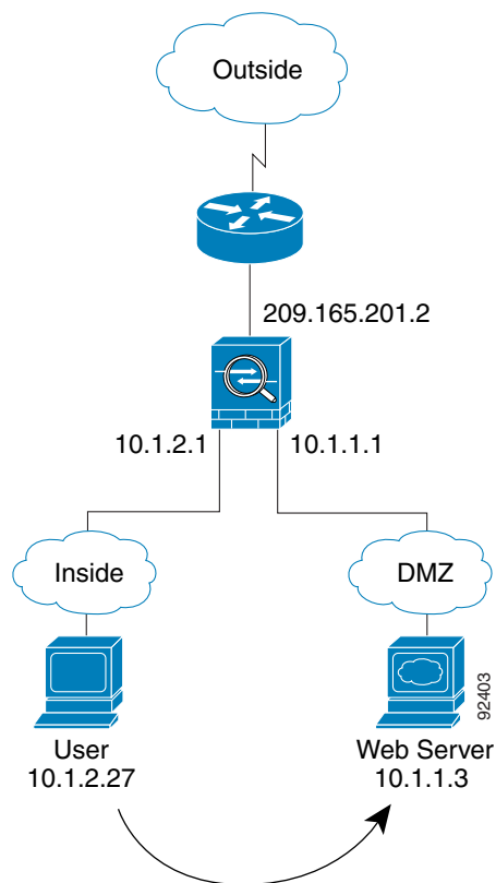
Figure 4-4 Inside to DMZ
