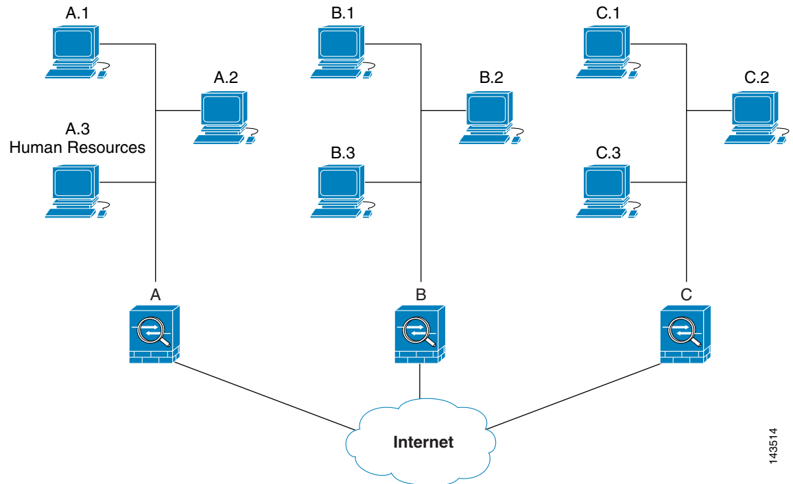
Figure 61-1 Effect of Permit and Deny ACEs on Traffic (Conceptual Addresses)
