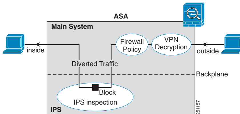
Figure 59-1 IPS Module Traffic Flow in the Adaptive Security Appliance: Inline Mode
