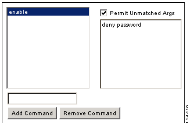
Figure 37-3 Disallowing Arguments
