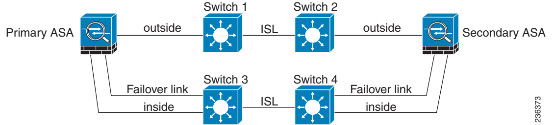
Figure 32-5 Connecting with a Secure Switch
