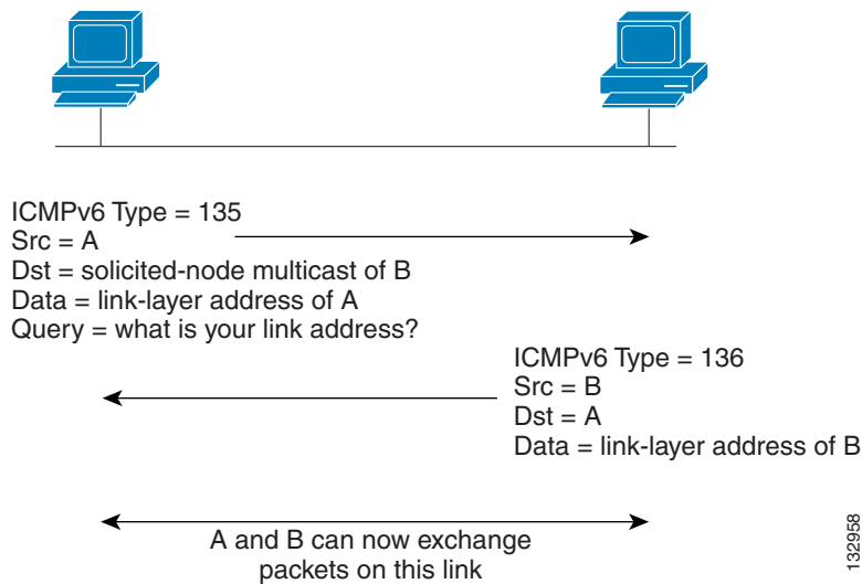
Figure 25-1 IPv6 Neighbor Discovery—Neighbor Solicitation Message
