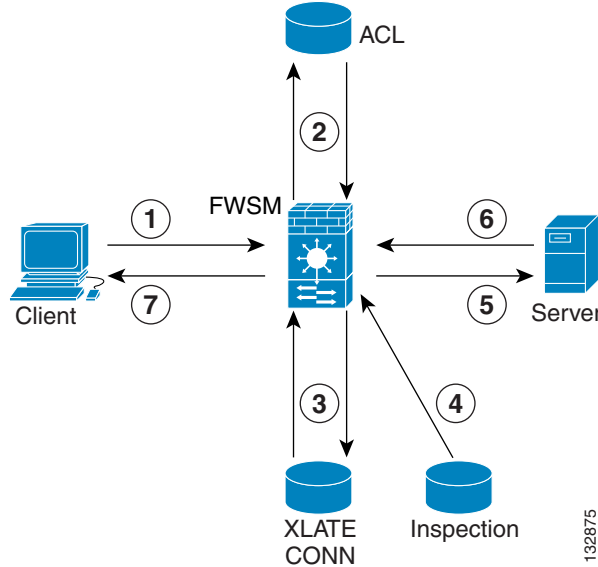
Figure 40-1 How Inspection Engines Work
