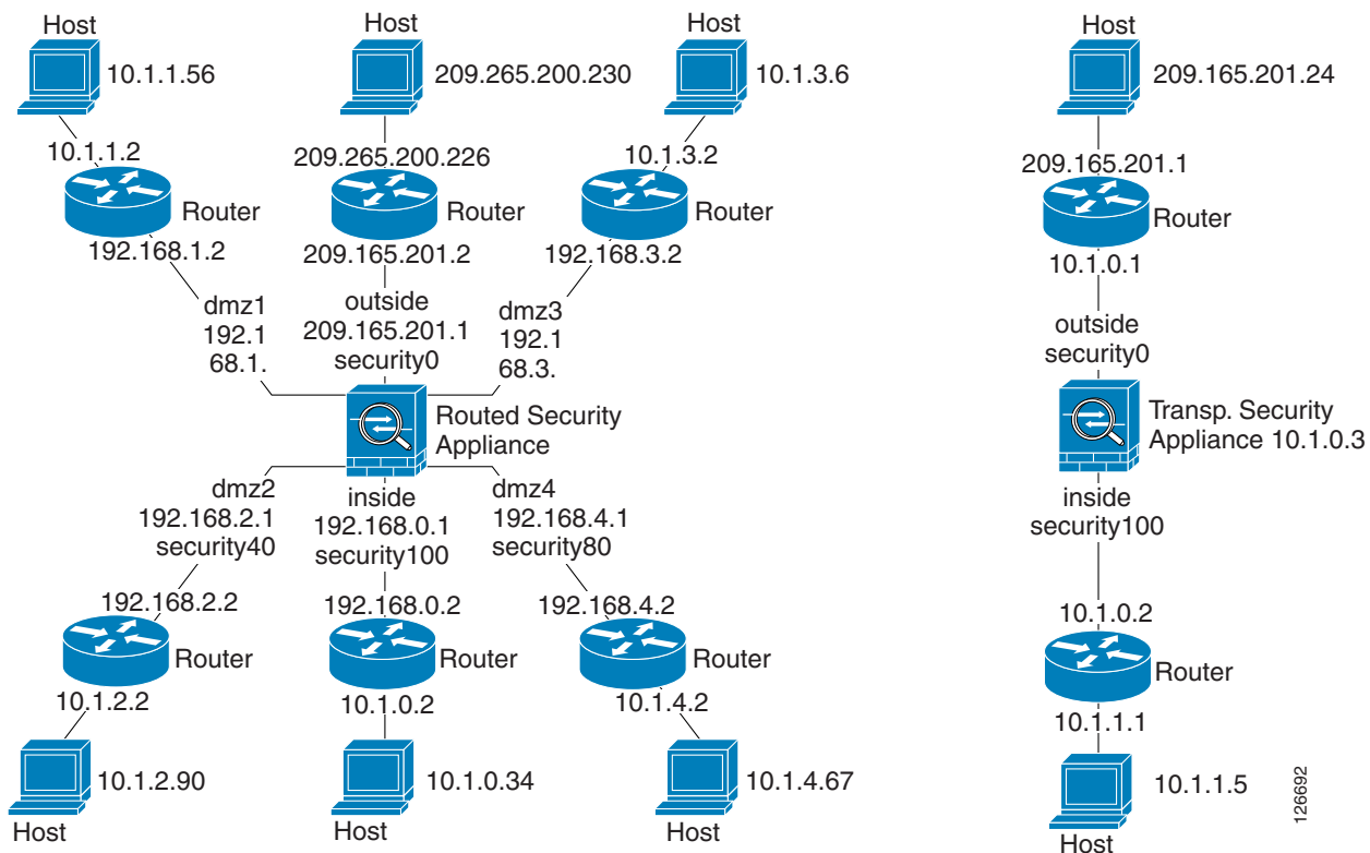
Figure 79-1 Network Diagram with Interfaces, Routers, and Hosts
