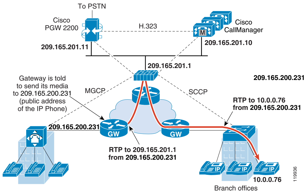
Figure 42-1 Using NAT with MGCP
