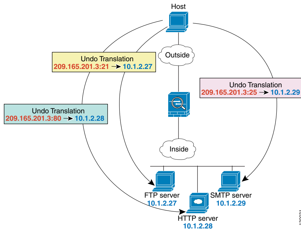
Figure 30-2 Static PAT
