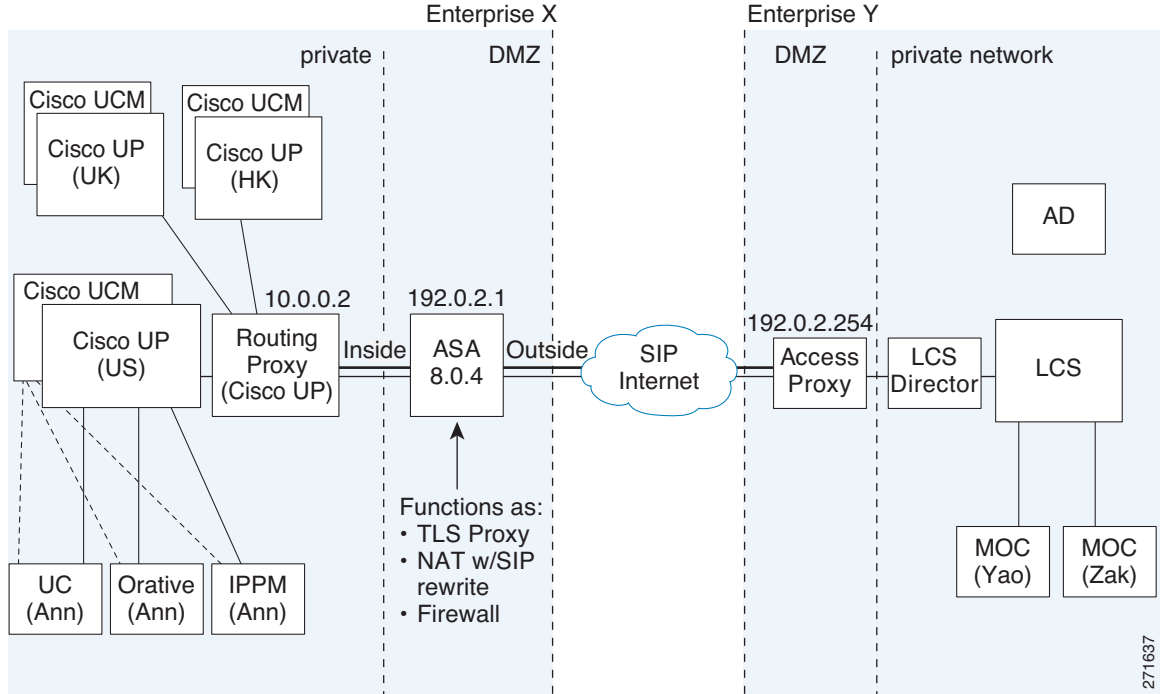
Figure 49-4 Typical Cisco Unified Presence/LCS Federation Scenario
