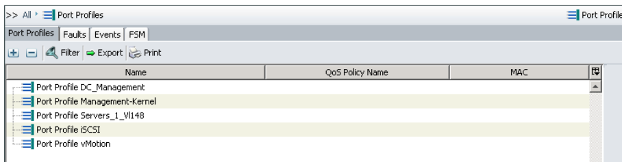
Figure 11 - Port profiles in Cisco UCS Manager
