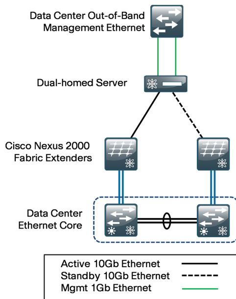
Figure 10 - Cisco UCS C-Series server with separate management interfaces
