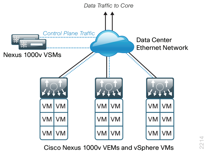
Figure 1 - Cisco Nexus 1000V logical view of control and VM traffic flow
