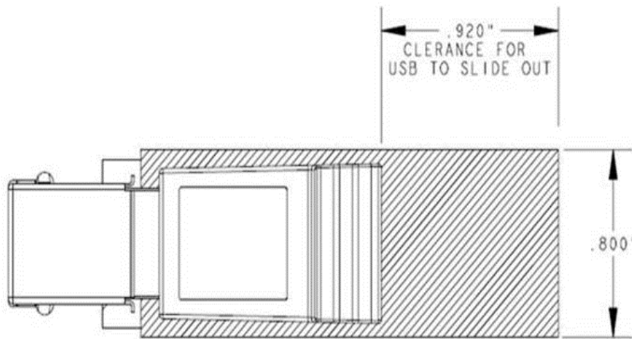
Figure 4 USB Clearance
