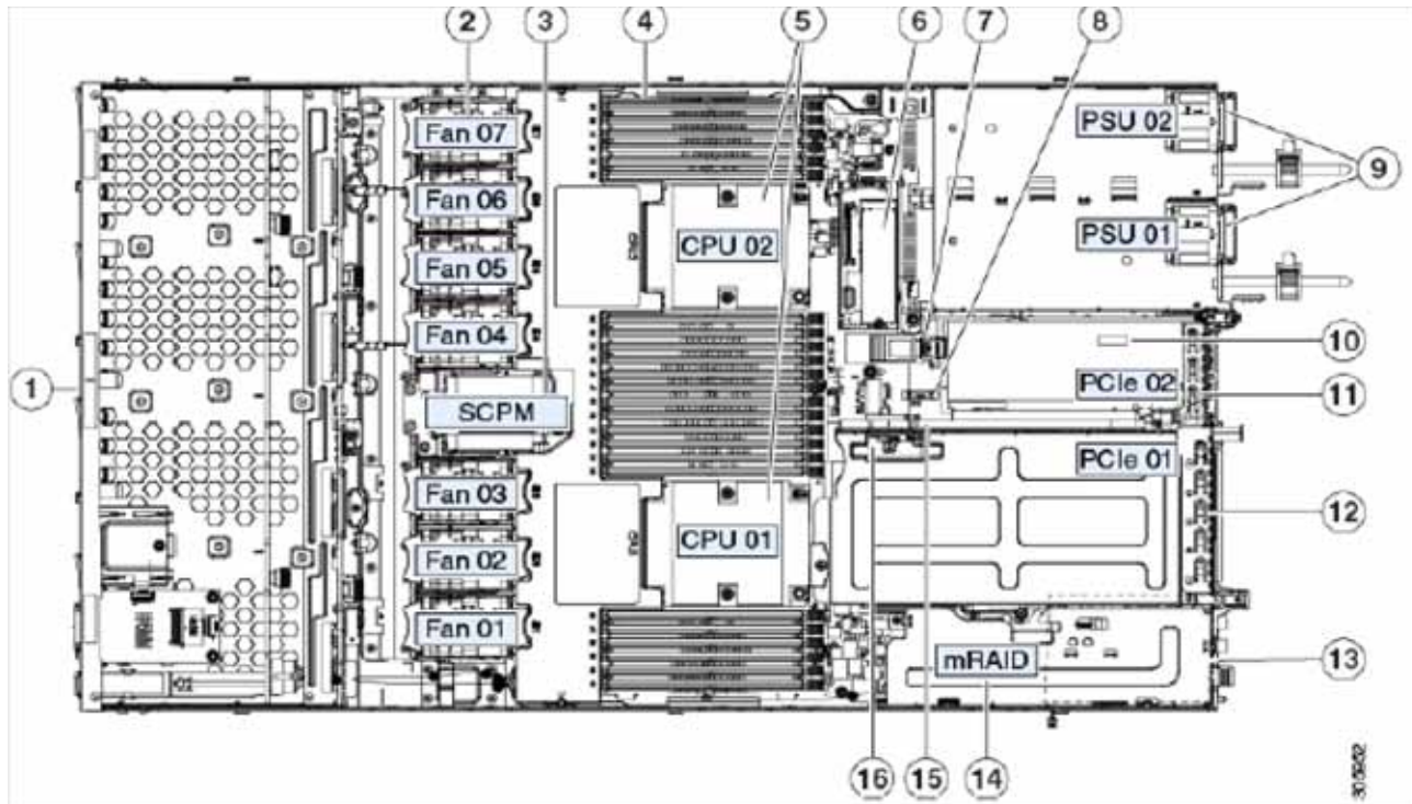
Figure 5 C220 M5 SFF With Top Cover Off
