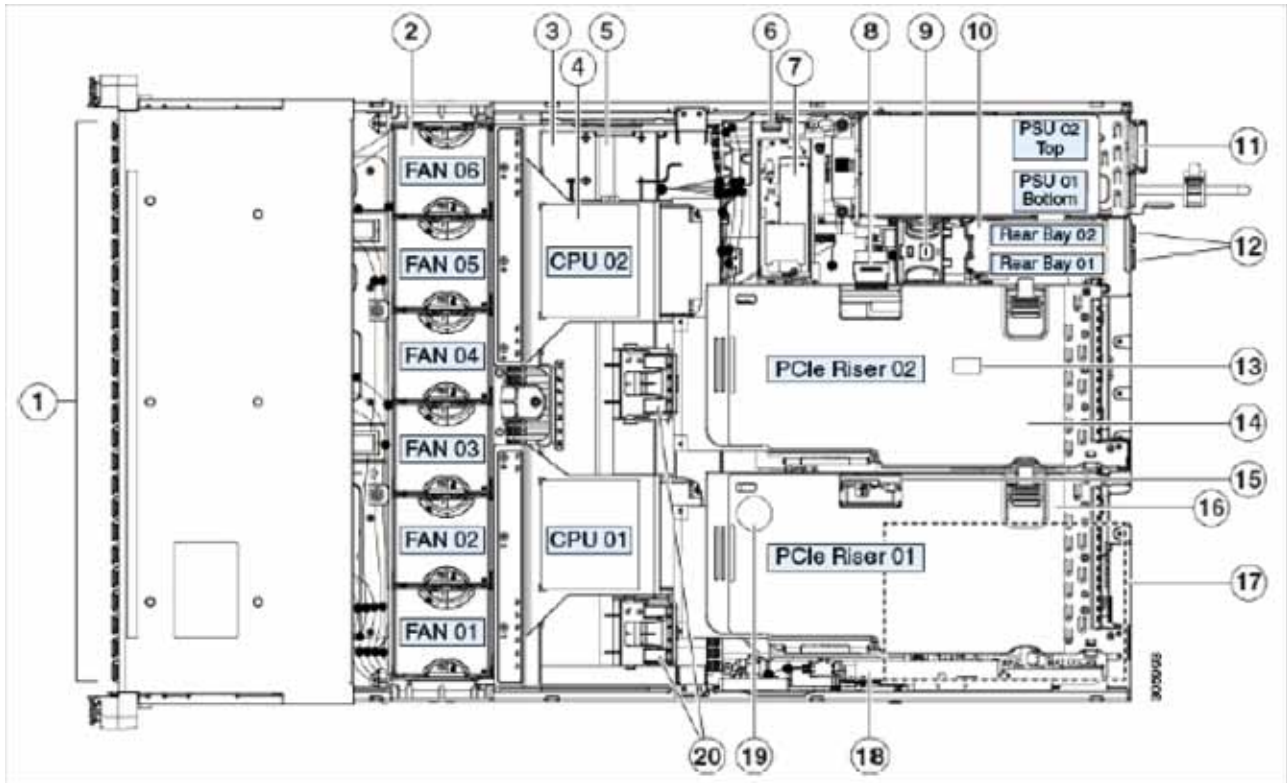
Figure 6 C240 M5 SFF With Top Cover Off
