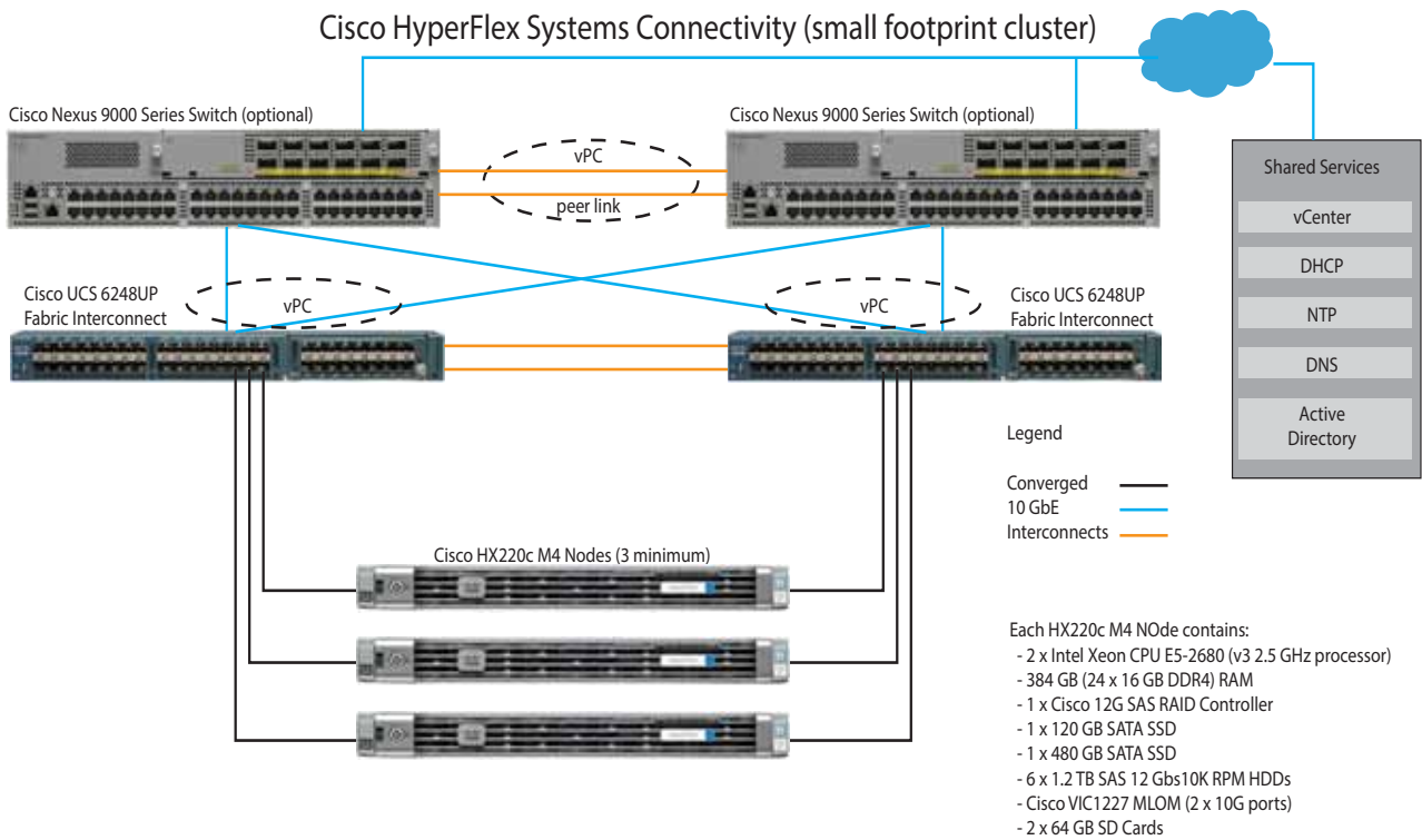
Figure 5 Small Footprint Cluster Using HX220c M4 Nodes
