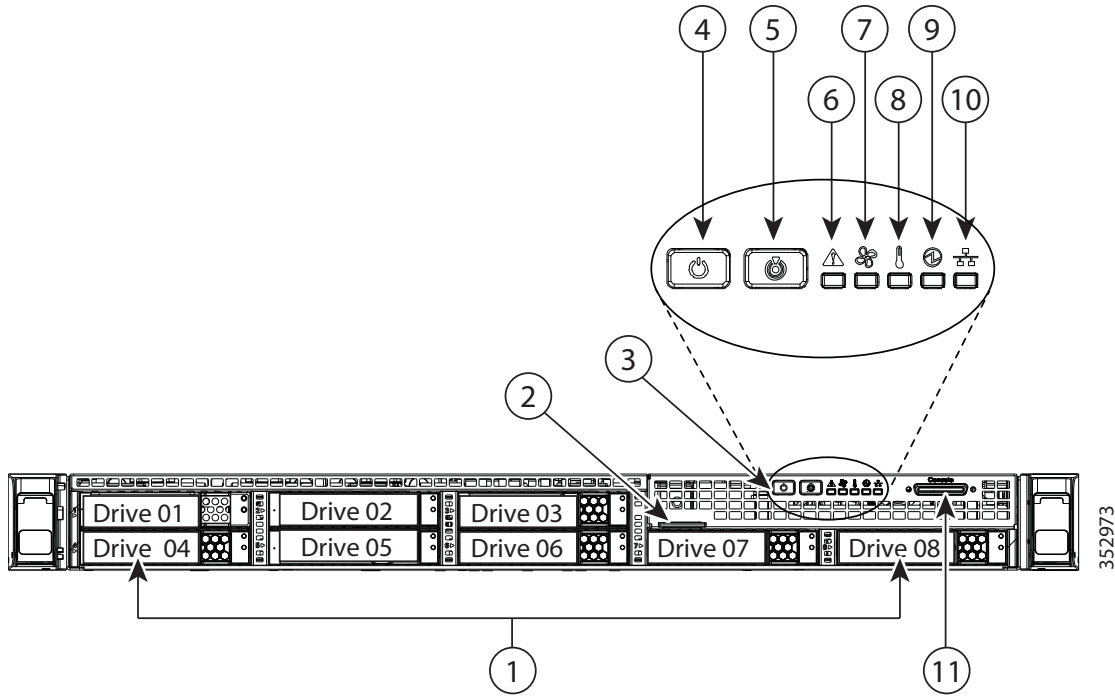
Figure 2 Chassis Front View
