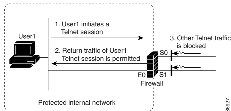
Figure 17 CBAC Opens Temporary Holes in Firewall Access Lists
