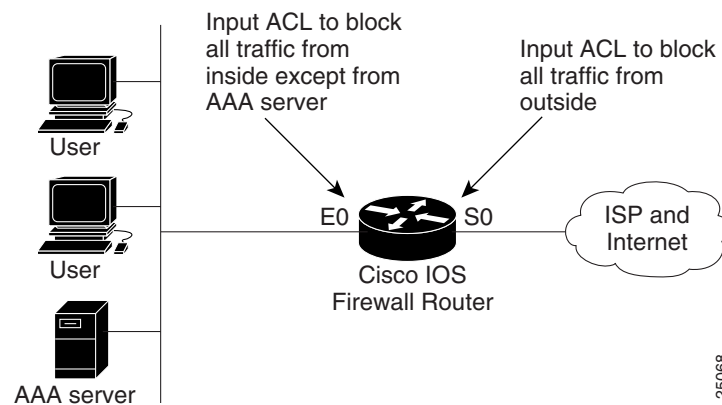
Figure 26 Applying the Authentication Proxy at the Local Interface
