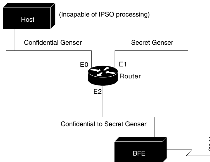
Figure 37 IPSO Security Levels
