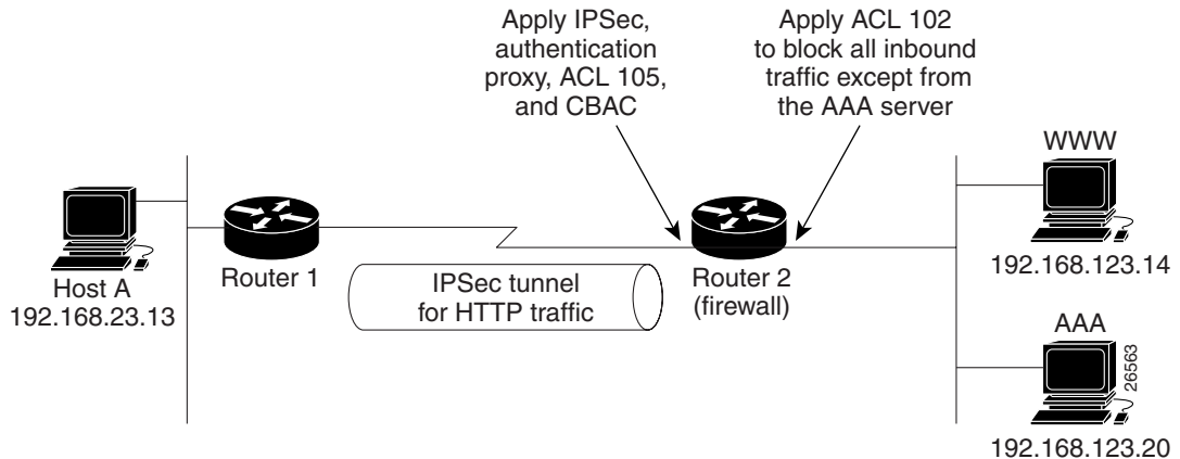
Figure 28 Authentication Proxy, IPSec, and CBAC Configuration Example
