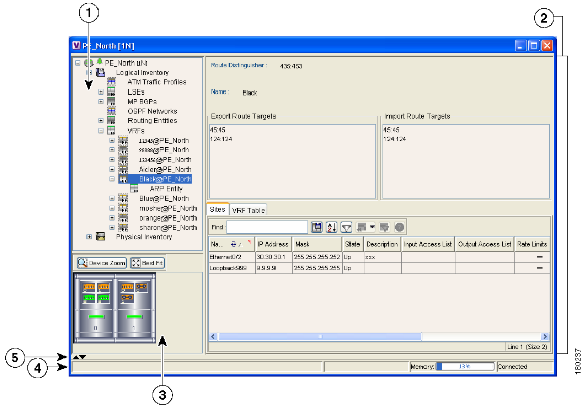
Figure 5-1 Inventory Window
