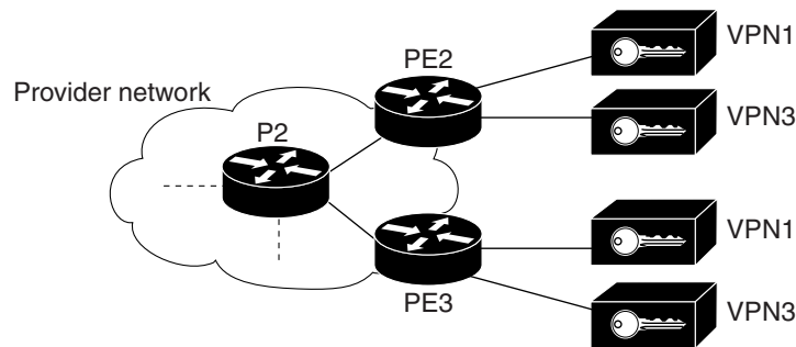
Figure 6-1 Example of a MPLS Black Hole Scenario
